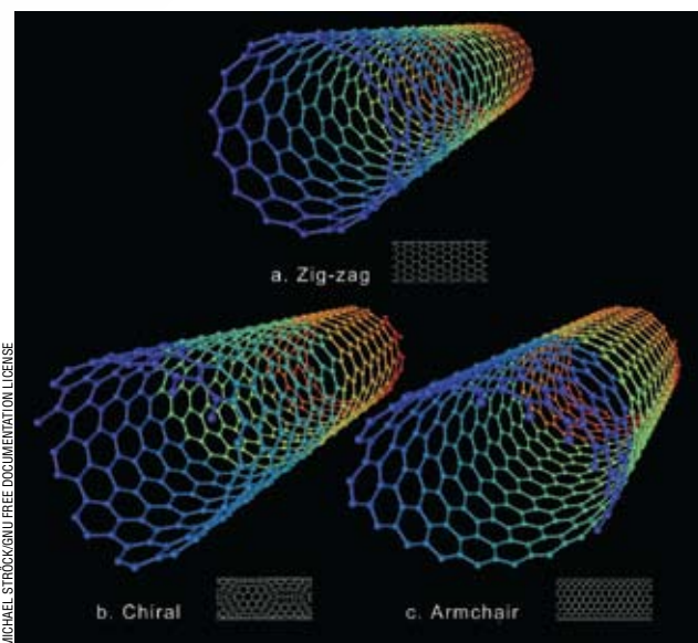
Figure 1. Structures of different types of carbon nanotubes: (a and c) Hexagons parallel to the axis of the tube; and (b) hexagons forming a helix that winds along the tube.
