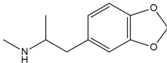
3,4-MethyleneDioxyMethAmphetamine
