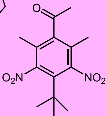
Musk ketone (synthetic musk)
