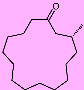
Muscone (musk deer glands)
