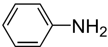
aniline
