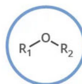
ETHER Naming: -oxy-ane e.g. methoxyethane
