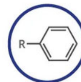
ARENE Naming: -yl benzene e.g. ethyl benzene
