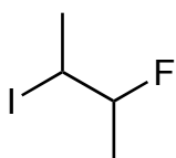
2-fluoro-1-iodo-1,2-dimethylethane
